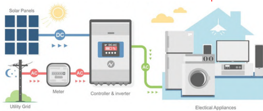
— On-grid Inverter working —
